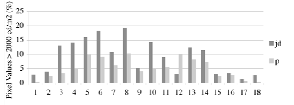
Figure 5: Percentage of pixel values that exceed a predetermined luminance threshold value of 2,000 \text{cd/m}^2
