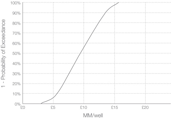
Figure 13: Subsea well P&A cost distribution: SNS
