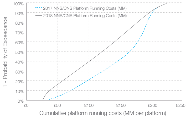
Figure 14: Change in platform running cost distribution: NNS & CNS
