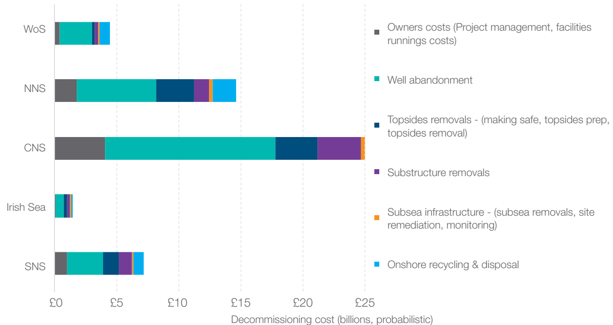
Figure 5: Decommissioning cost distribution by category
